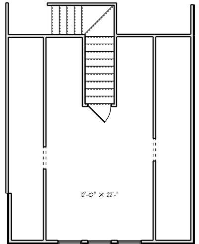
BONUS ROOM FLOOR PLAN SCALE: 1" = 1/4"
