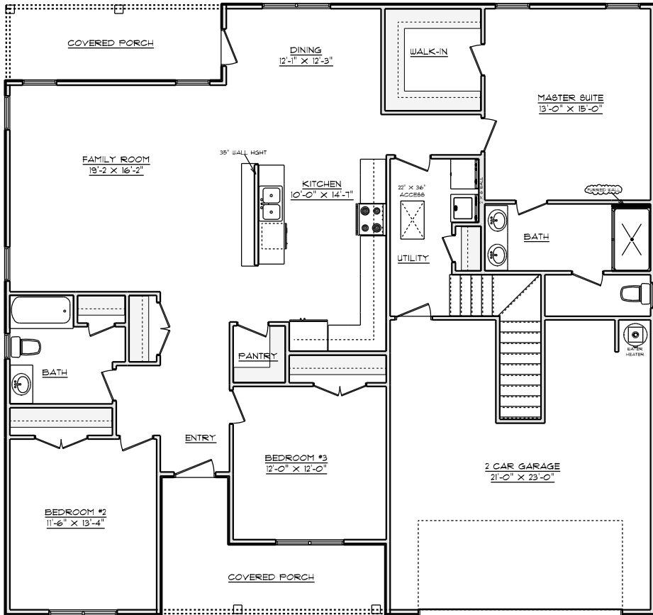
FLOOR PLAN SCALE: 1" = 1/4"
